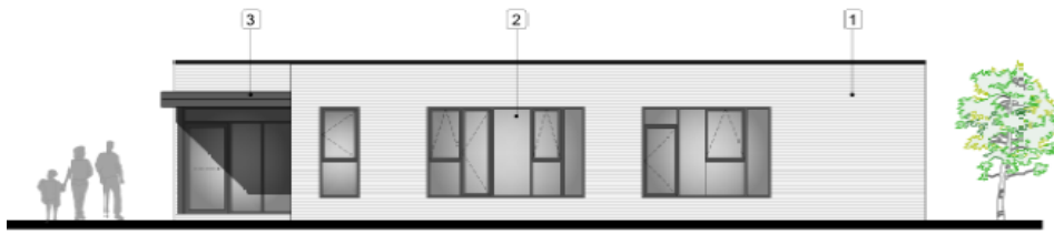
ELEVATION 1 SOUTH
